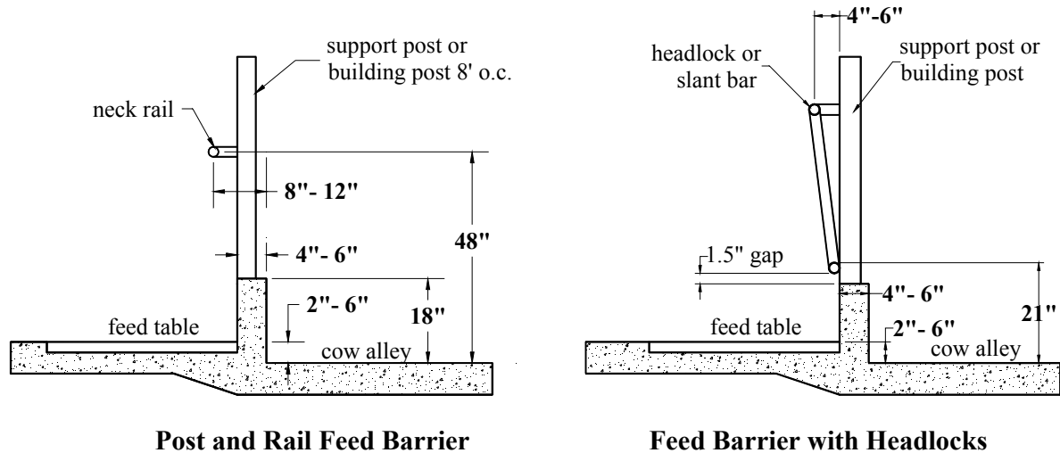
Figure 1. Typical feed barrier types and dimensions for mature Holstein cows (1,400 lb) .
