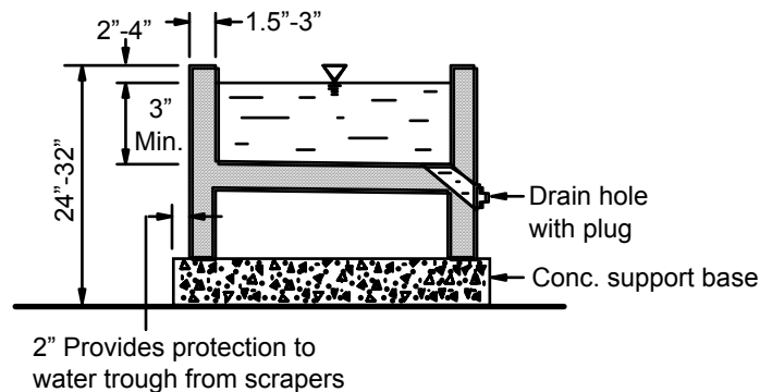
Figure 3. Cross section of concrete or polyethylene water trough (Graves, et al., 1997).
